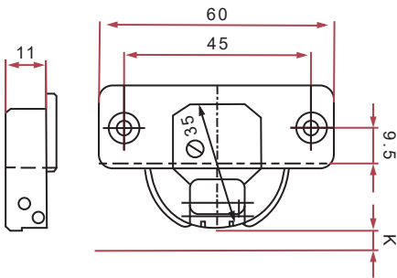
Drilling for cup
