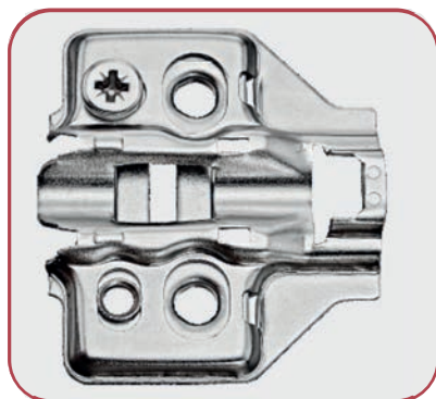
Cruciform plate with cam and pre-assembled euro screws
