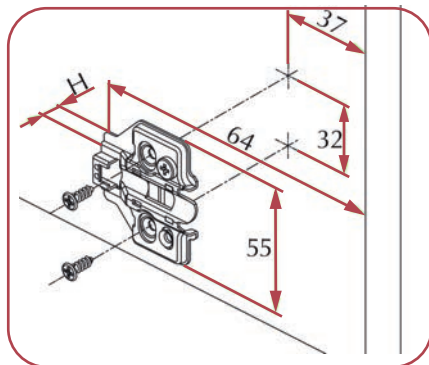
Cruciform plate with cam and pre-assembled euro screws
