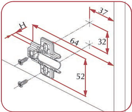
Cruciform plate with pre-assembled euro screws
