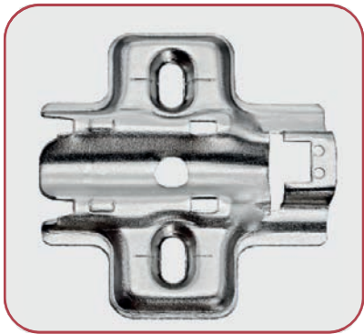
Cruciform plate with pre-assembled euro screws
