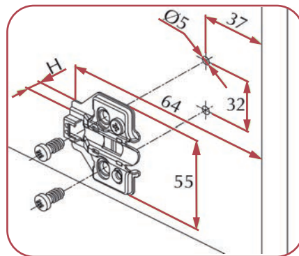
Cruciform plate with pre-assembled 5mm diameter cam shanks
