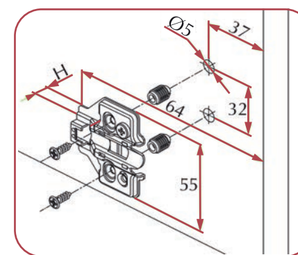
Cruciform plate with pre-assembled 10mm diameter cam shanks
