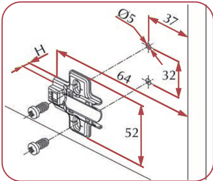
Cruciform plate with pre-assembled 5mm diameter shanks
