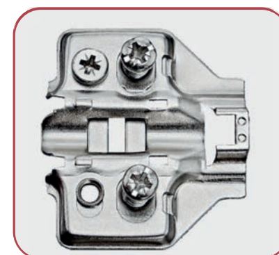
Cruciform plate with pre-assembled 10mm diameter cam shanks
