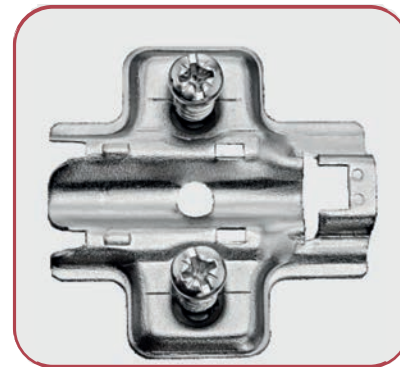
Cruciform plate with pre-assembled 10mm diameter shanks
