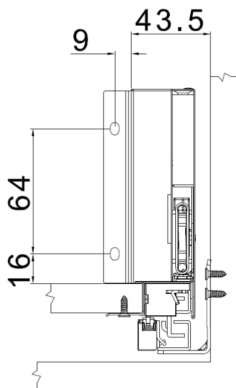
back panel mounting position
