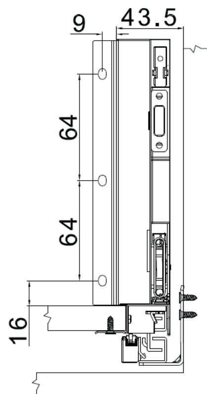
back panel mounting position
