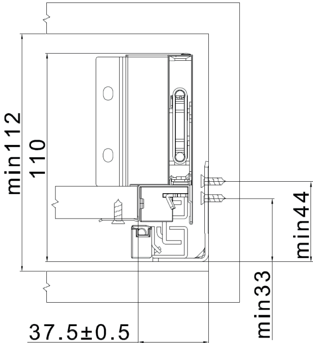
internal cabinet size
