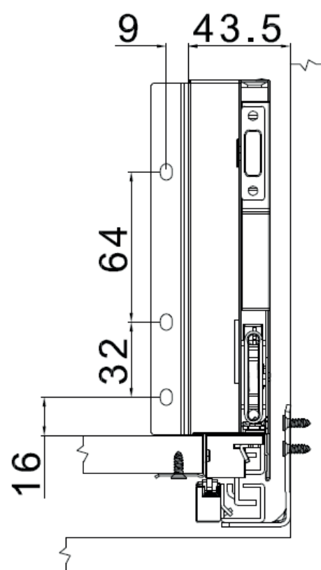
back panel mounting position
