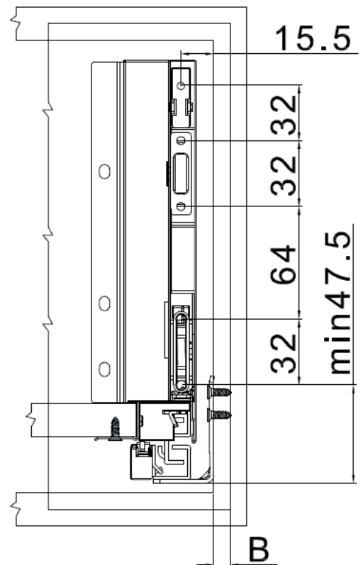
front panel mounting position
